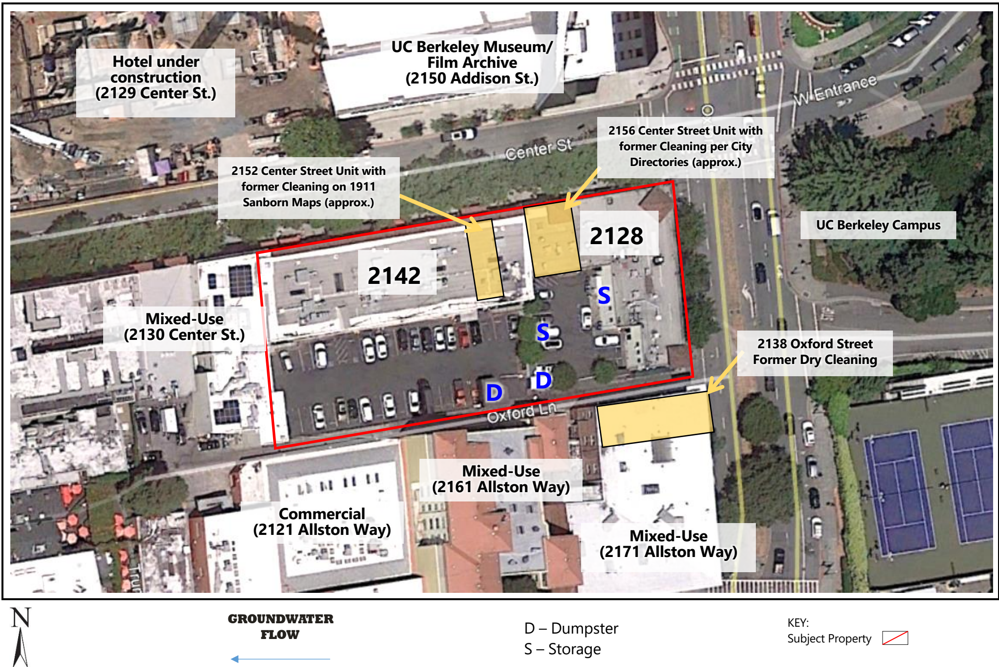
FIGURE 2: SITE PLAN Project No. 20-297761.2
